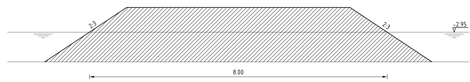
DETAIL DAM SCHAAL 1:50
